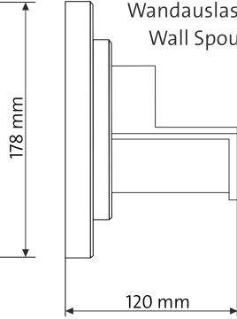
Wandauslass Ellipse Wall Spout Ellipse
